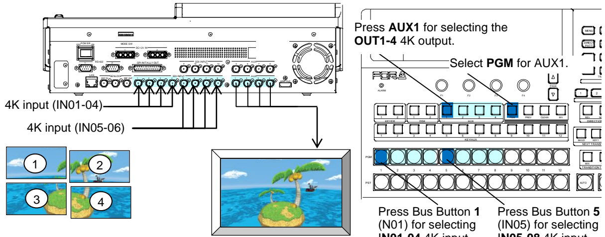
Control panel
