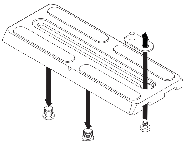
Fig. 7 Fitting the 1/4 in. pin adaptor assembly
