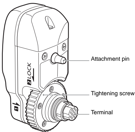
Transmitter Case
