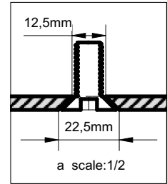
Flat head socket cap screw DIN7991 M10X25
