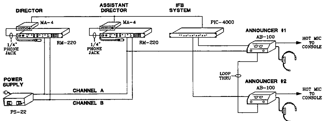
AB-100 Connected To A Clear-Com Party-line System
