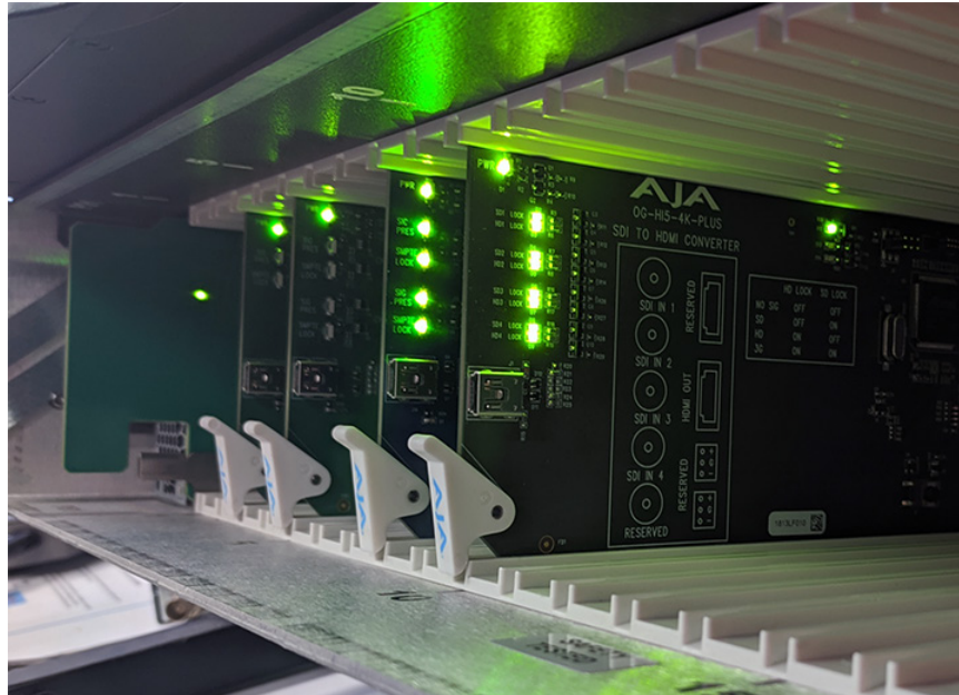
Figure 8. The white plastic tab for the card second from the right is now upright. All cards are shown fully inserted.
