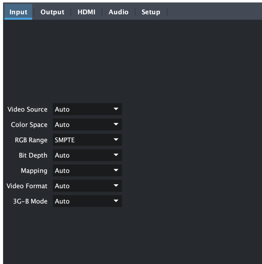
Figure 13. OG-4K2HD Input Tab Screen in DashBoard
