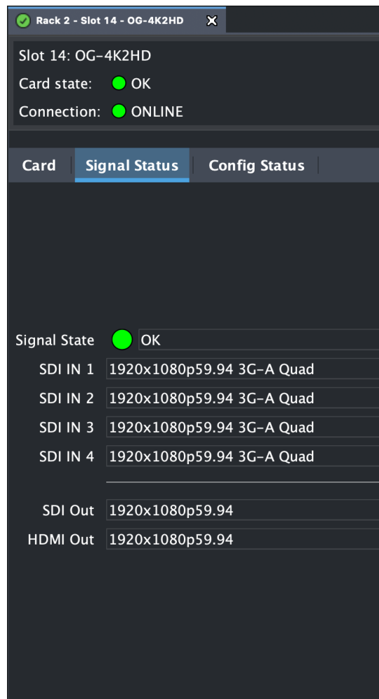
Figure 11. OG-4K2HD Signal Status Tab Screen in DashBoard
