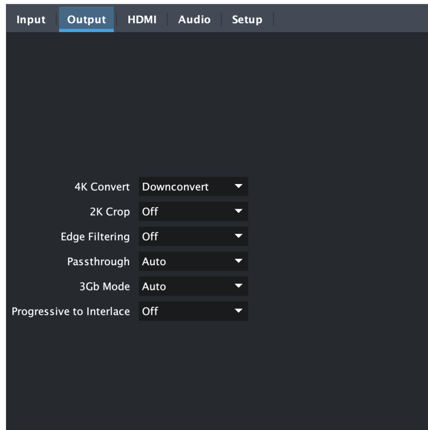
Figure 14. OG-4K2HD Output Tab Screen in DashBoard
