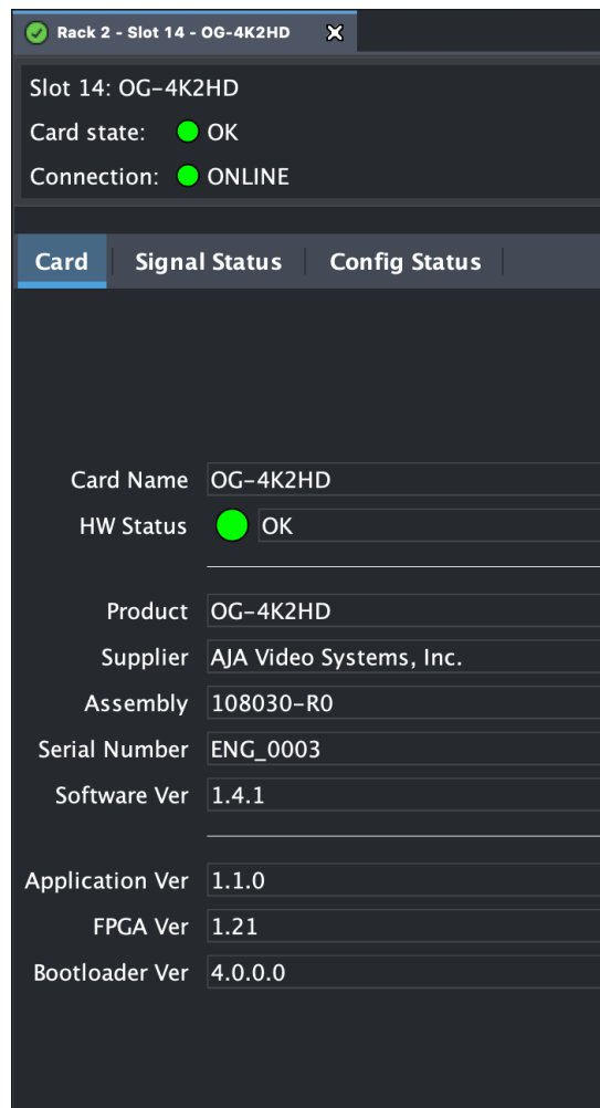
Figure 10. OG-4K2HD Card Tab Screen in DashBoard
