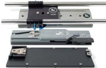
QuickLock Adapter Kit 401-F231 for Sony F23 / F35, base plates replaces the original Sony base plates.
