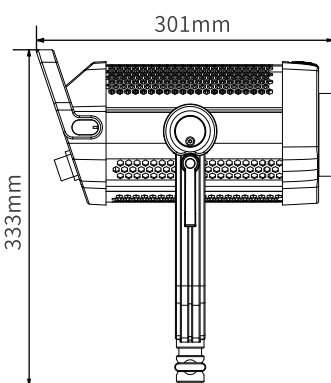
Fig.2 BL-300 Left View
