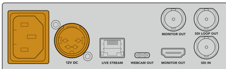
Web Presenter HD can be powered using the IEC or 12V DC power input
