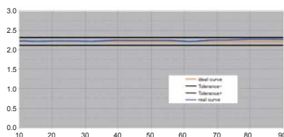
Diagram 1: Gamma curve between 10% and 90% signal level. Blue line (real curve) indicates the monitor.
