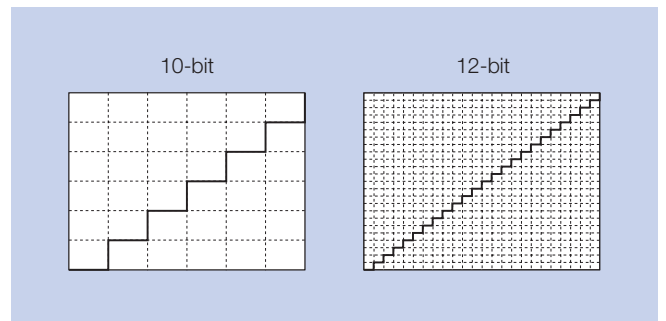
fig 2 High-Intergrity 12-bit A/D Conversion
