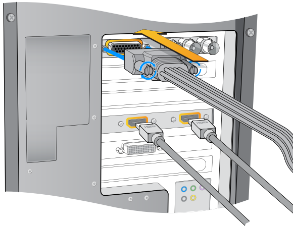
Attach the supplied DeckLink breakout cable to the DeckLink card. The DeckLink HD Extreme 3 card also includes a HDMI bracket as pictured above.
