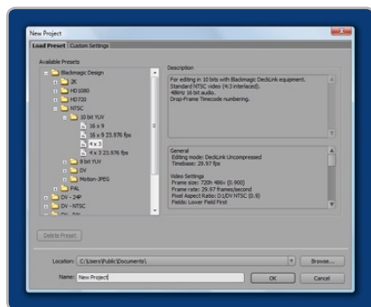
New Project.
