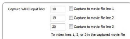
VANC preferences.
