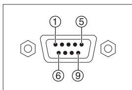
D-sub 9-pin (male) Serial output
