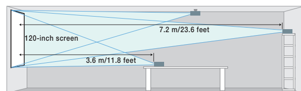
NOTE: This illustration shows the projection distances of the PT-F300NTE/F300E.
