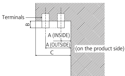
Terminal a 80BF1 Terminal (Bottom)
