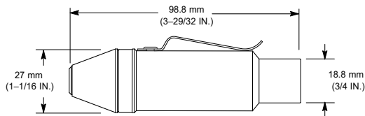
SM93 PREAMPLIFIER
