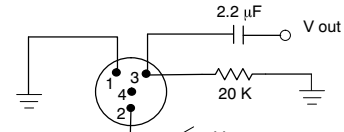
TEST CIRCUIT FIGURE 3
