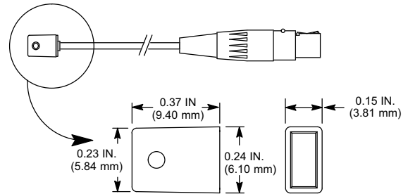
SM93/WL93 MICROPHONE
