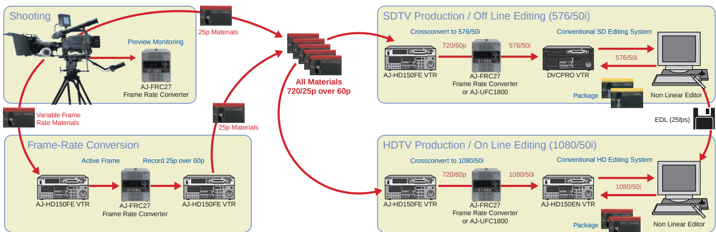
System Flow-Chart for TV Programme Production (25-fps)
