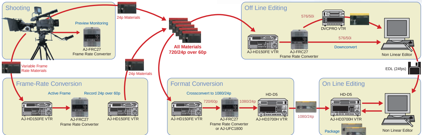
System Flow-Chart for Cinema Production (24-fps)
