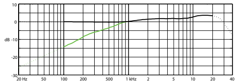
Frequency Response of d:fine™ Directional
