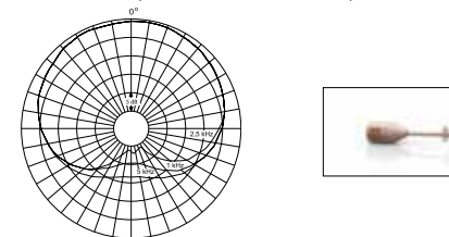
Polar Pattern (d:fine™ 4088 and d:fine™ 88)
