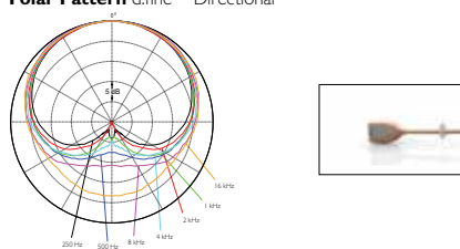
Polar Pattern d:fine™ Directional
