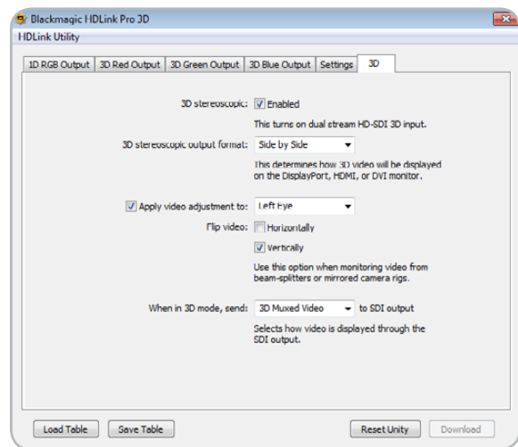
3D pane in Windows
