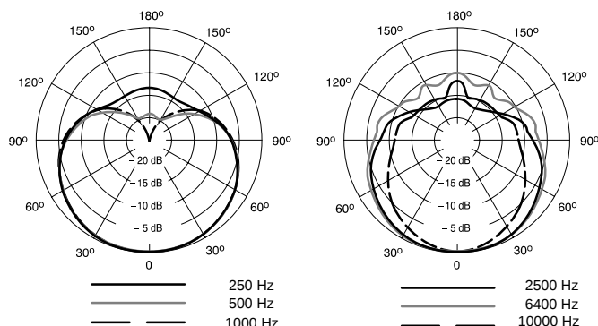
POLAR PATTERNS
