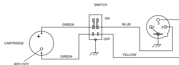
INTERNAL CONNECTIONS
