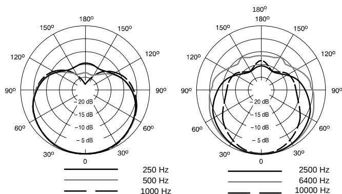
POLAR PATTERNS
