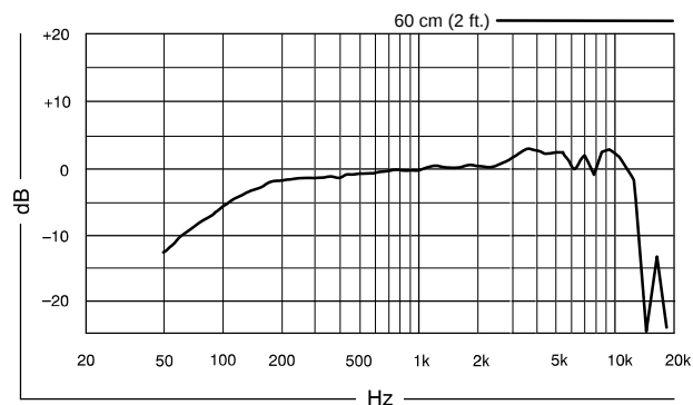
FREQUENCY RESPONSE
