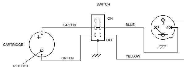
INTERNAL CONNECTIONS
