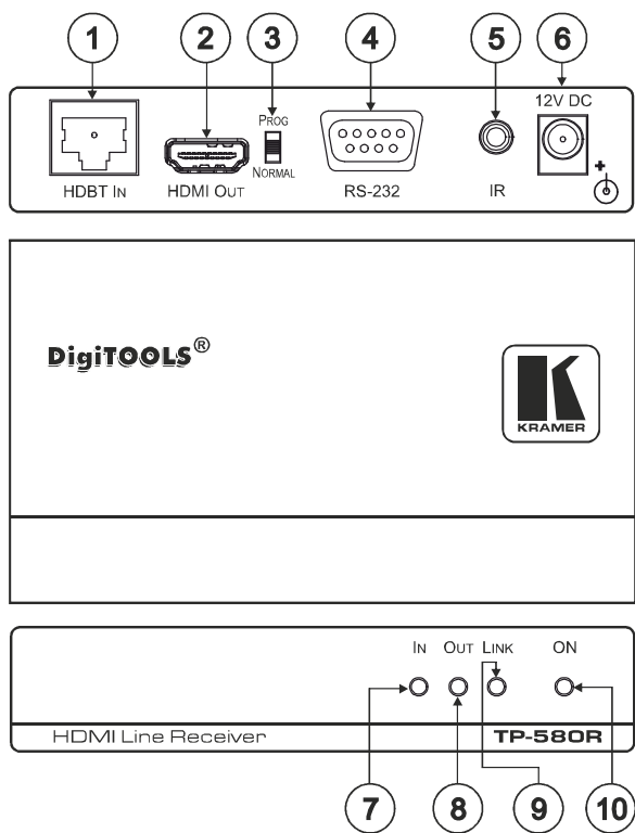
Figure 2: TP-580R HDMI Line Receiver
