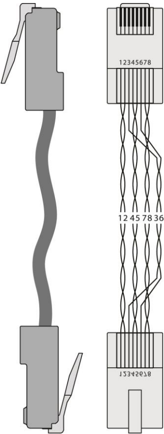
Figure 9: TP PINOUT
