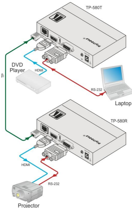
Figure 7: RS-232 Control
